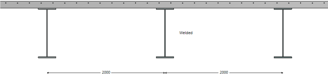
Figure 8 : Transversal view
