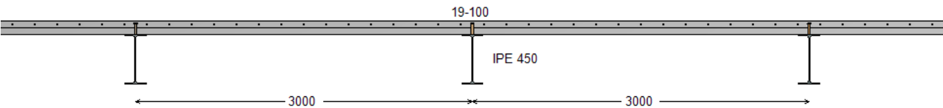
Figure 2 : Transversal view
