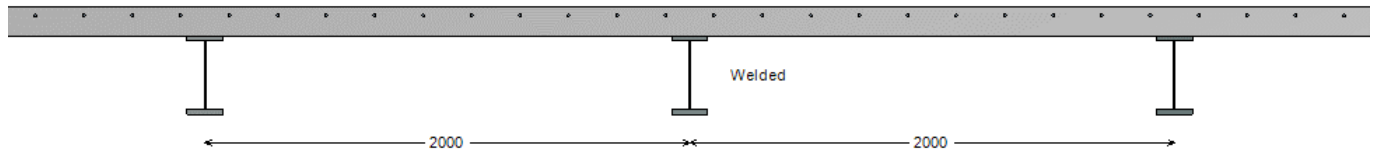
Figure 11 : Transversal view
